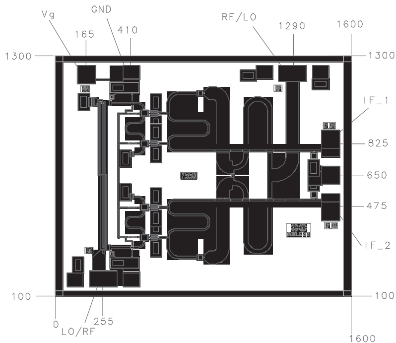
Figure 13. Bond pad location (um)
